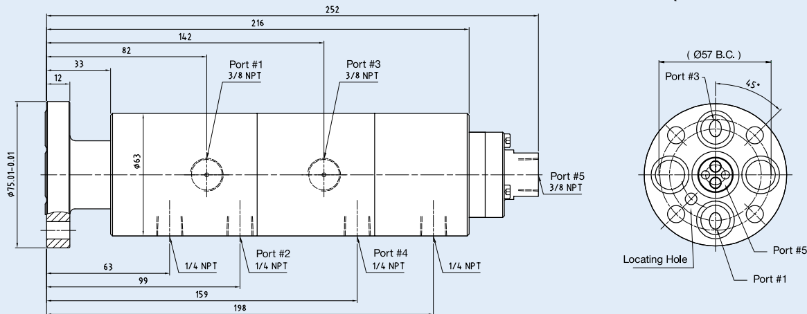
End View (2630-100-001 shown)
