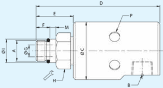
Radial Connection
