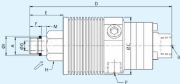
Axial Connection
