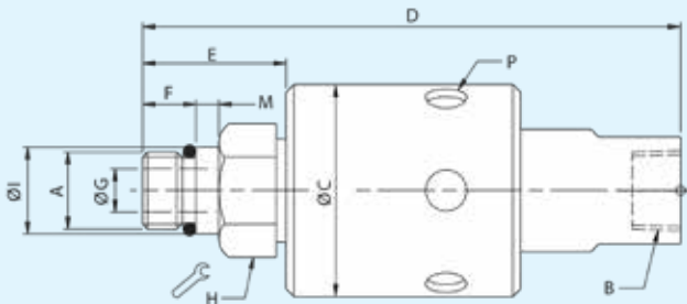
Axial Connection
