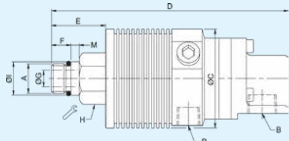
Radial Connection
