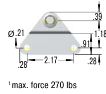
OG8-V4A Side Bracket
