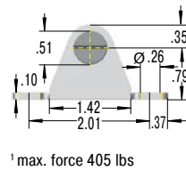
MA10 Bearing Shoe
