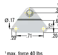
OG5-V4A Side Bracket
