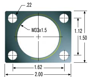
250-0293 Rectangular Flange
