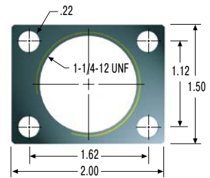
250-0016 Rectangular Flange
