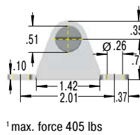
MA10-V4A Bearing Shoe
