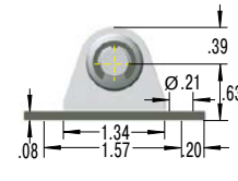
NA8-V4A Angle Bracket
