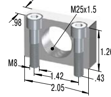
250-0436 Mounting Block
