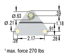
OE10 Side Bracket
