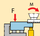
Figure 5c Correctly located workpiece
