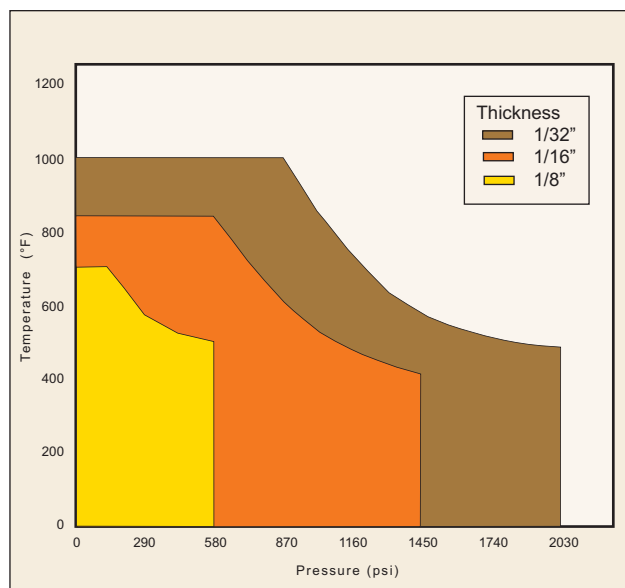
Flexitallic Thermiculite® 715 Pressure/Temperature Curve - Temperature and pressure guides cannot be used simultaneously and do not apply to all thicknesses. In keeping with Industry norm, Flexitallic suggests that cut gaskets be limited to Class 300 service max unless fully confined in a groove.
