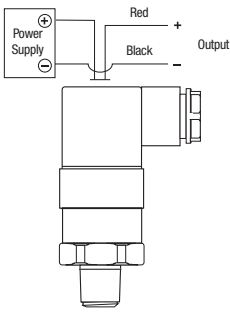
2 WIRE WIRING DIAGRAM EXAMPLE
