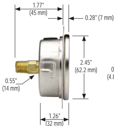
25-911 Front Flange
