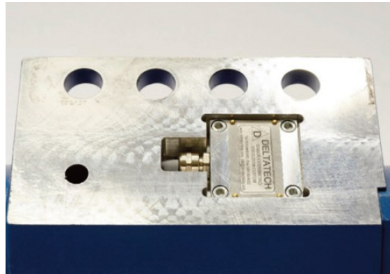
Protected Mounting Location on AF1470 Sensors
