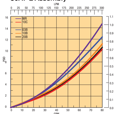
80AT-2 Assembly
